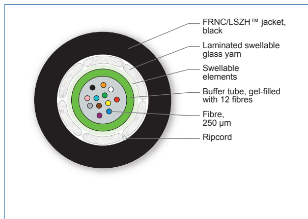
Cross Section of Order Number: 012TEU-13188A2G
